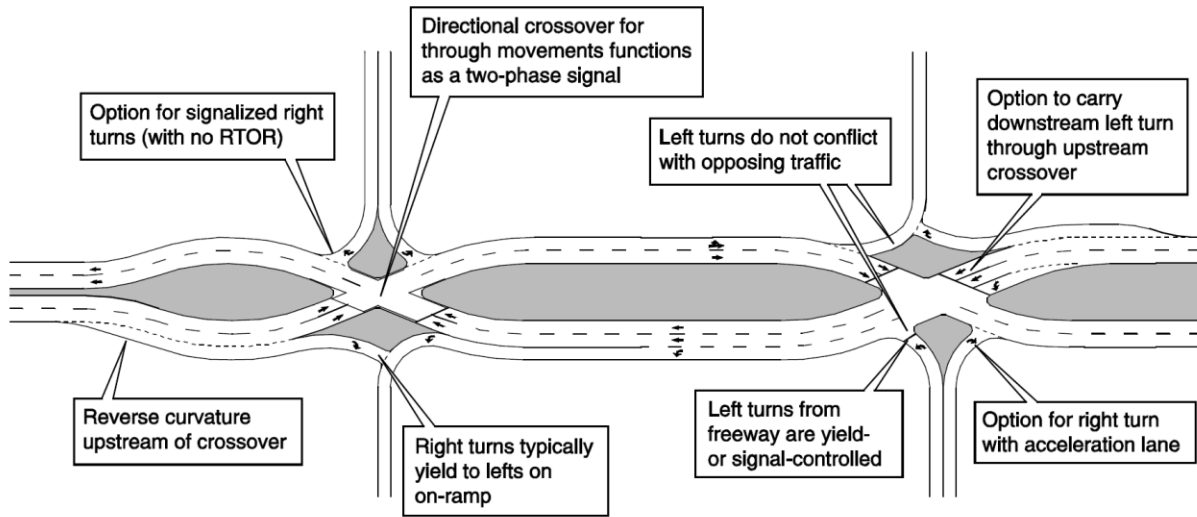
Figure 6-4 Example of a DDI intersection and its key characteristics
