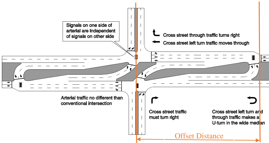
(a) Example of a RCUT Intersection with signal
