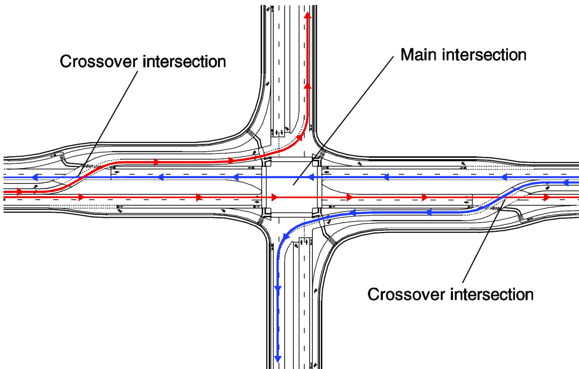
Figure 6-5 Example of a DLT intersection design sketch
